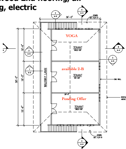
SECOND FLOOR PLAN SCALE: 1/8"=1'-0"
